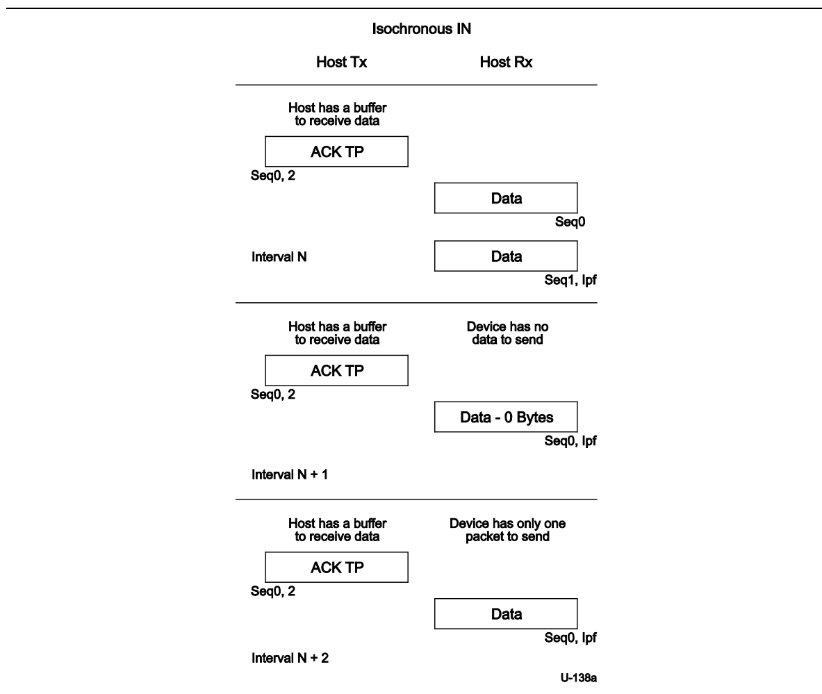
Figure 8-62. Sample Enhanced SuperSpeed Isochronous IN Transaction
