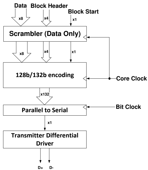
Gen 2 transmitter
