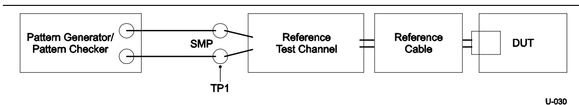
Figure 6-27. Rx Tolerance Setup
