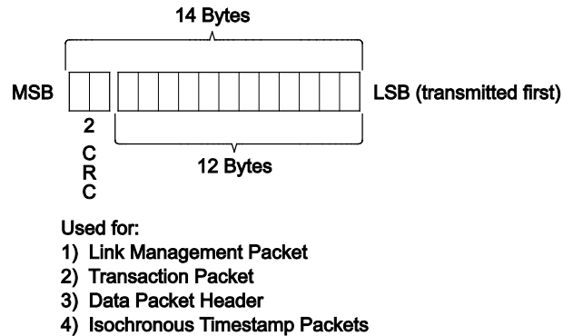
Figure 7-5. Packet Header
