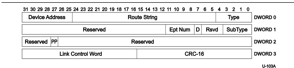
Figure 8-21. STATUS Transaction Packet
