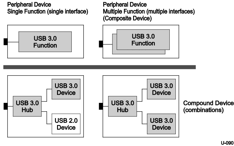
Figure 3-5. Examples of Supported USB 3.1 USB Physical Device Topologies
