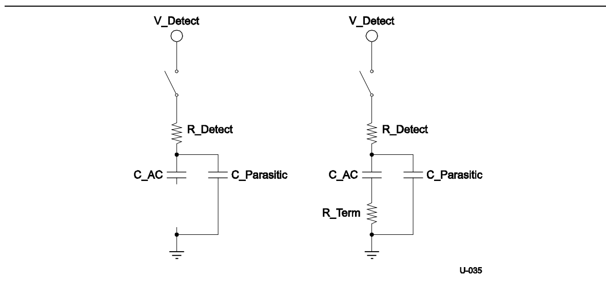
Figure 6-36. Rx Detect Schematic
