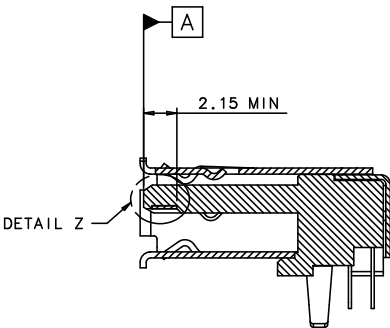
SECTION J-J
