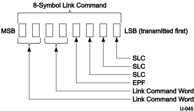
Figure 7-12. Link Command Structure
