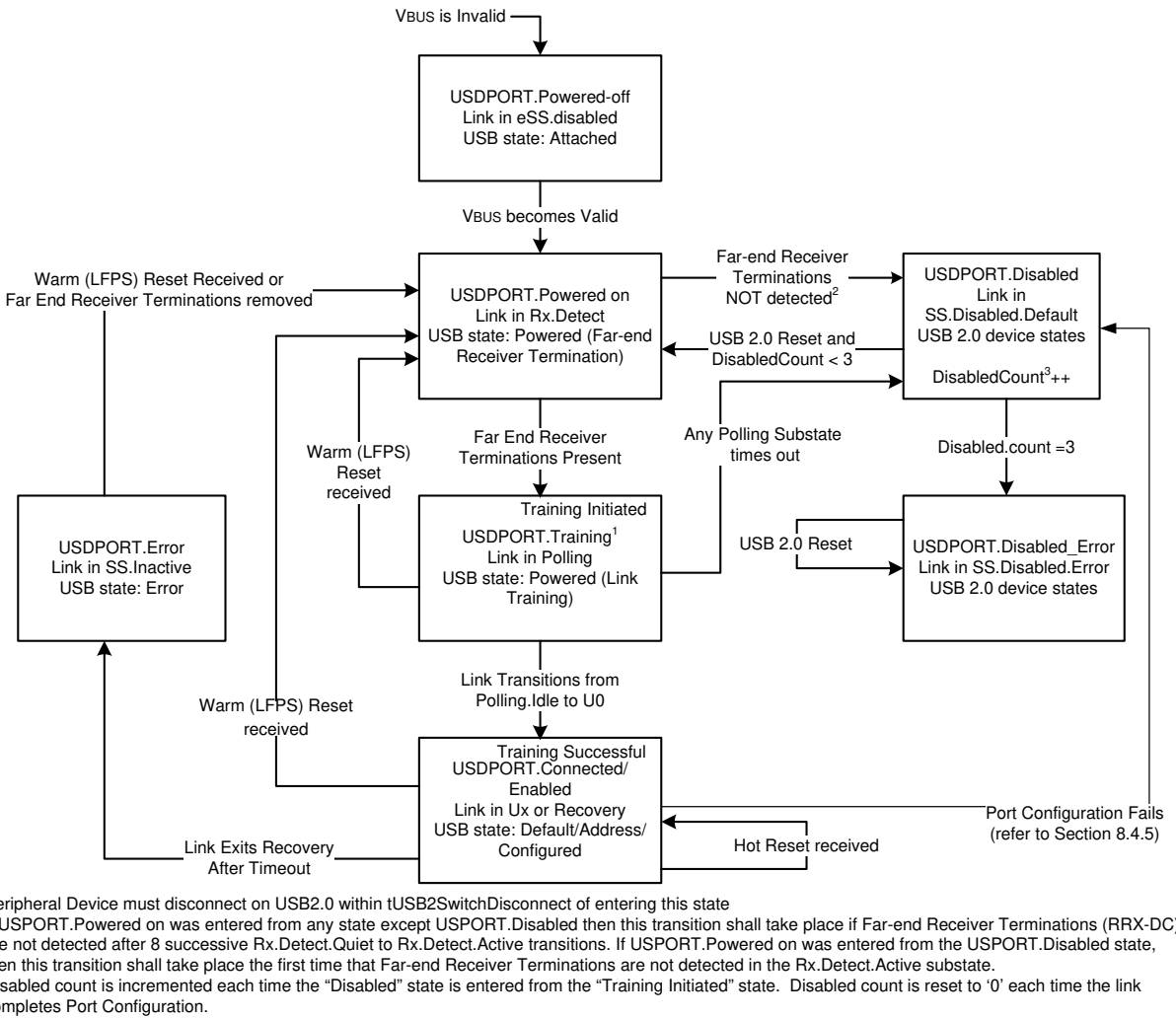
Figure 10-26. Peripheral Upstream Device Port State Machine
