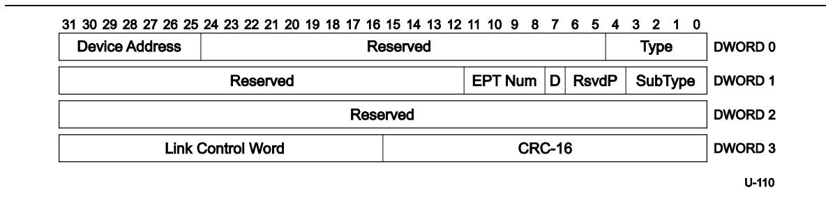
Figure 8-29. PING_RESPONSE Transaction Packet
