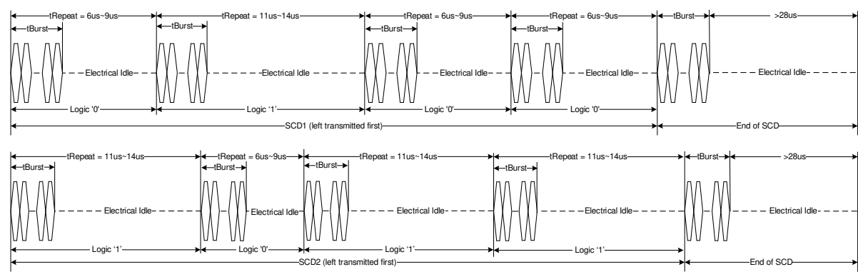
Figure 6-33. SCD1/SCD2 transmission
