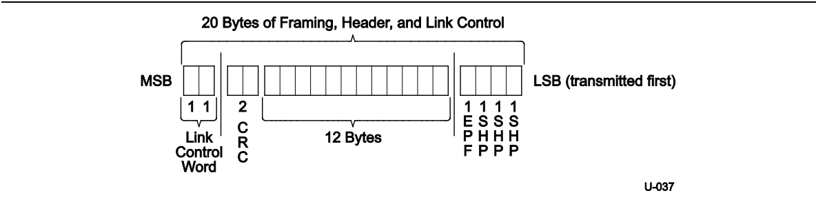
Figure 7-3. Enhanced SuperSpeed Header Packet with HPSTART, Packet Header, and Link Control Word
