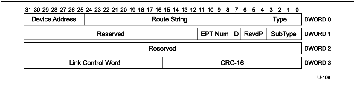
Figure 8-28. PING Transaction Packet
