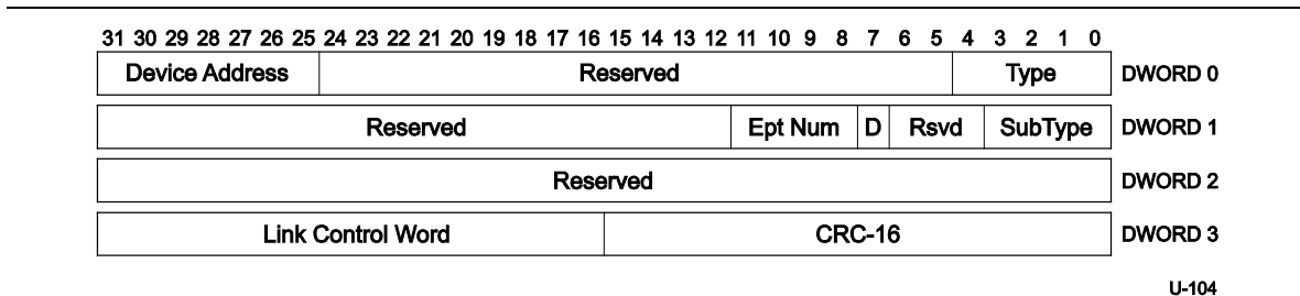
Figure 8-22. STALL Transaction Packet
