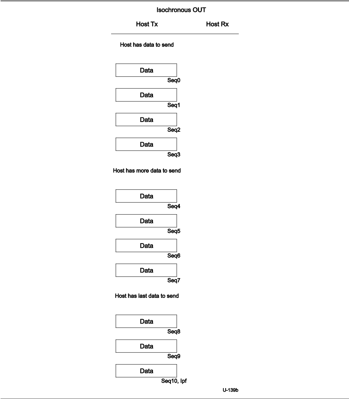
Figure 8-65. Sample Enhanced SuperSpeed Isochronous OUT Transaction
