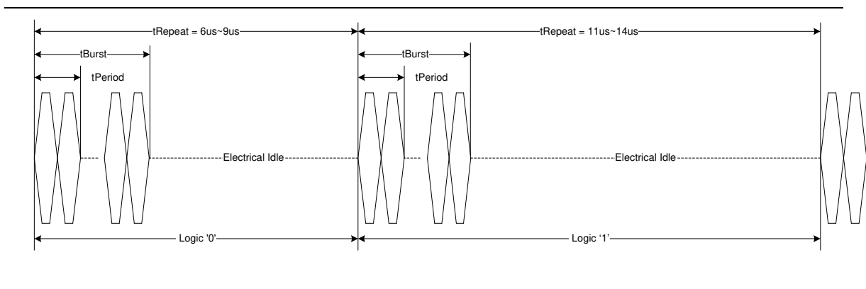
Figure 6-32. Example of Binary Representation based on Polling.LFPS
