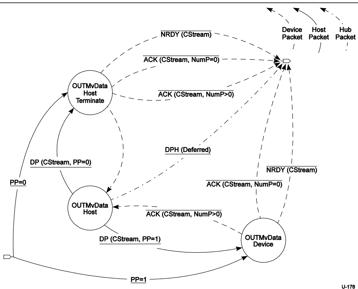
Figure 8-42. Device OUT Move Data State Machine (DOMDSM)
