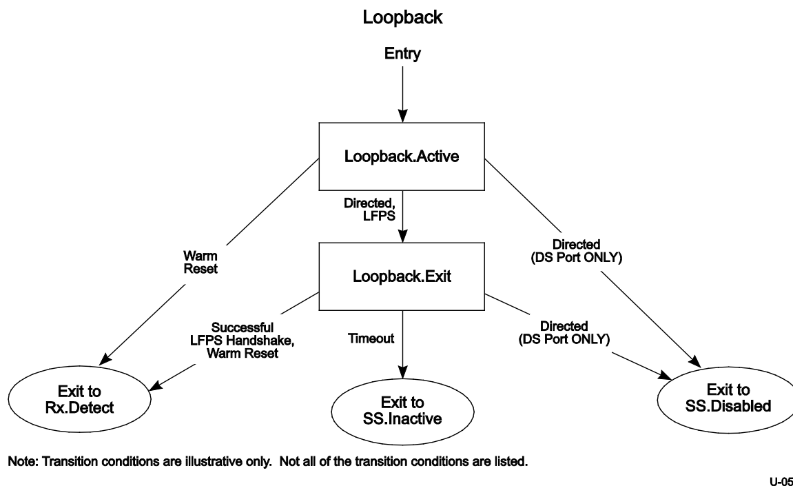
Figure 7-23. Loopback Substate Machine
