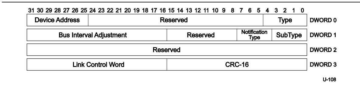
Figure 8-26. Bus Interval Adjustment Message Device Notification
