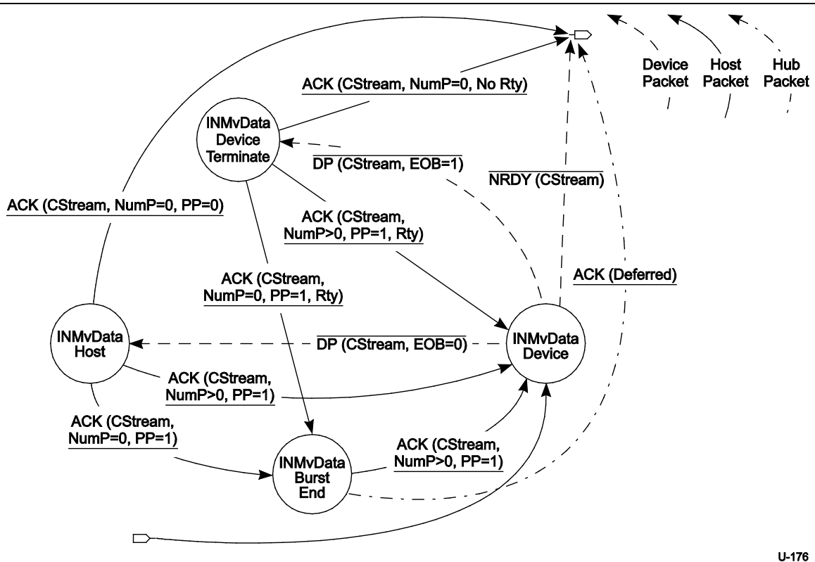
Figure 8-40. Device IN Move Data State Machine (DIMDSM)
