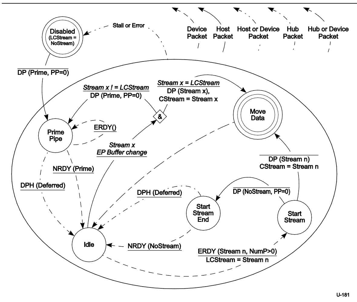
Figure 8-45. Host OUT Stream Protocol State Machine (HOSPSM)
