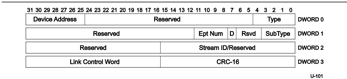
Figure 8-19. NRDY Transaction Packet
