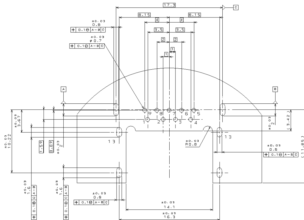
Figure 5-6. Example Footprint for the USB 3.1 Standard-A Receptacle - Mid-Mount Standard Mount Through-Hole with Insertion Detect
