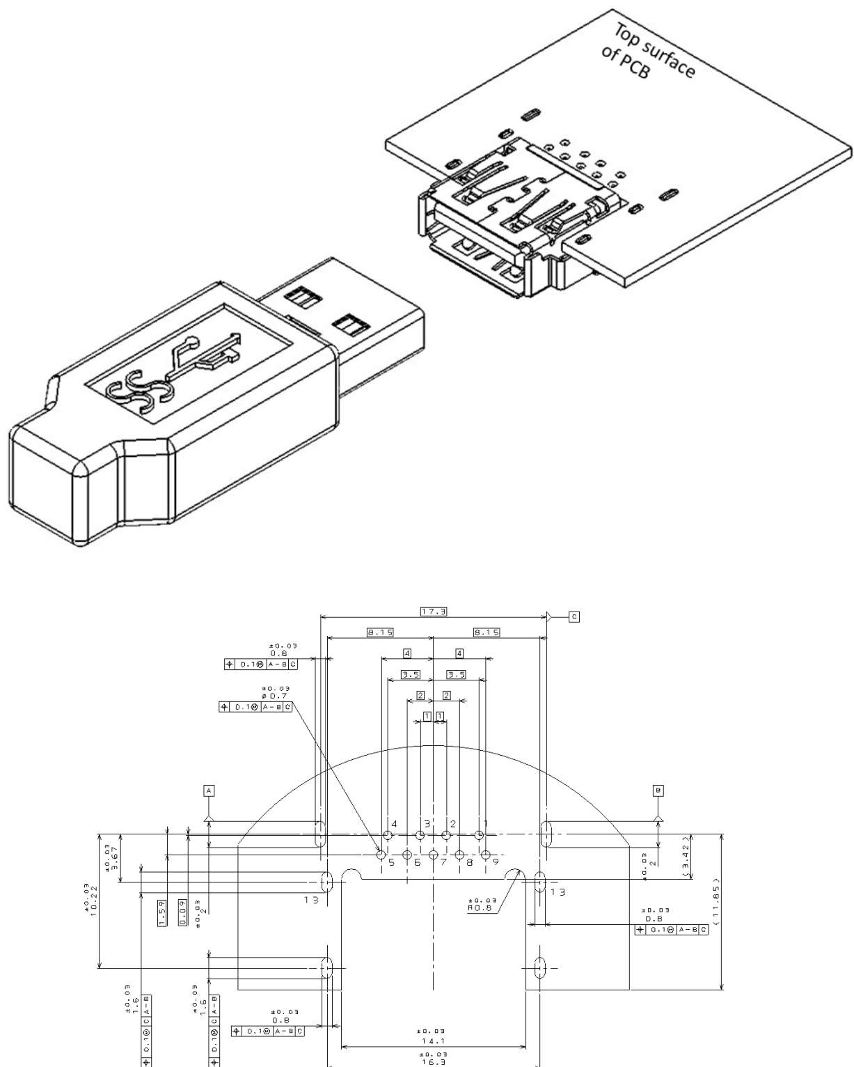
Figure 5-7. Example Footprint for the USB 3.1 Standard-A Receptacle - Mid-Mount Reverse Mount Through-Hole with Insertion Detect
