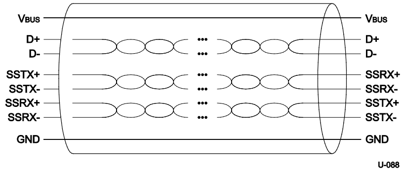
Figure 3-2. USB 3.1 Cable
