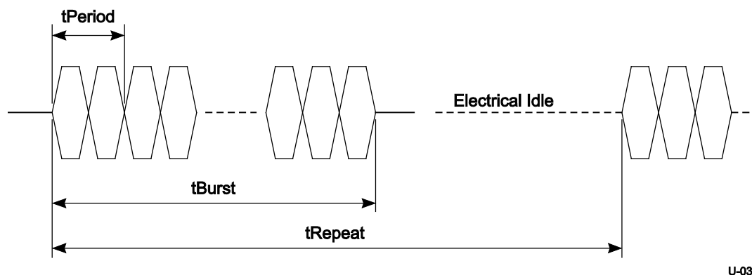
Figure 6-29. LFPS Signaling
