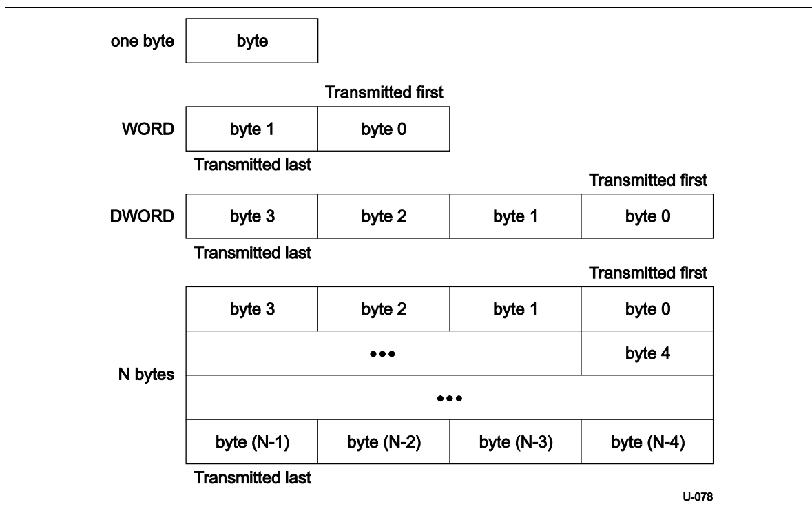
Figure 7-2. Byte Ordering
