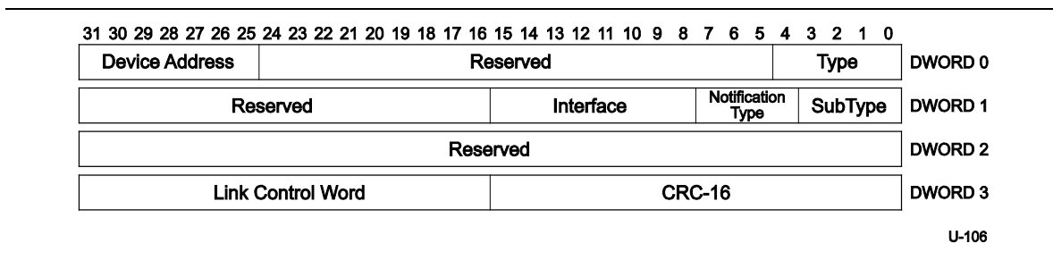
Figure 8-24. Function Wake Device Notification
