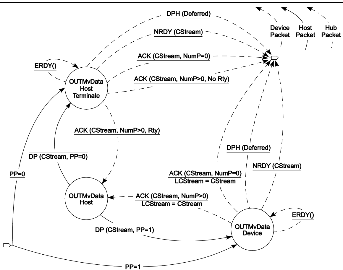
Figure 8-46. Host OUT Move Data State Machine (HOMDSM)
