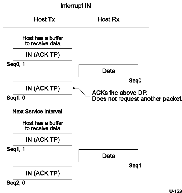
Figure 8-49. Host Sends Interrupt IN Transaction in Each Service Interval
