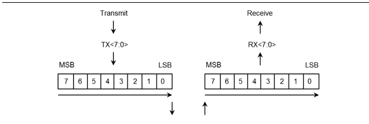
Figure 6-9. Gen 2 Serialization and Deserialization Order
