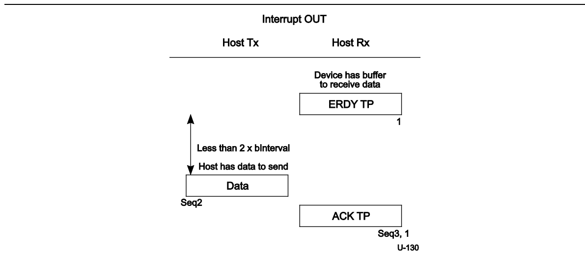
Figure 8-56. Host Resumes Sending Interrupt OUT Transaction After Device Sent ERDY
