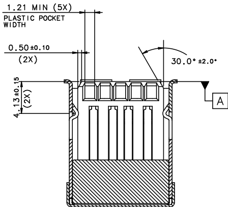
SECTION S-S
