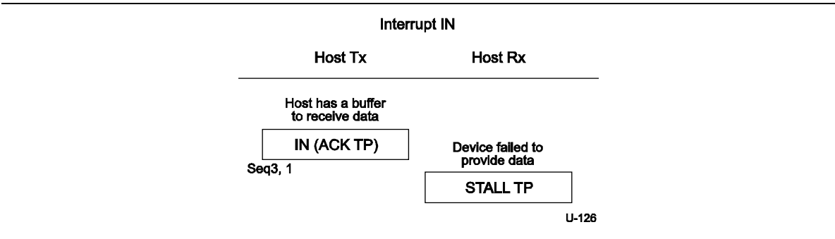
Figure 8-52. Endpoint Sends STALL TP
