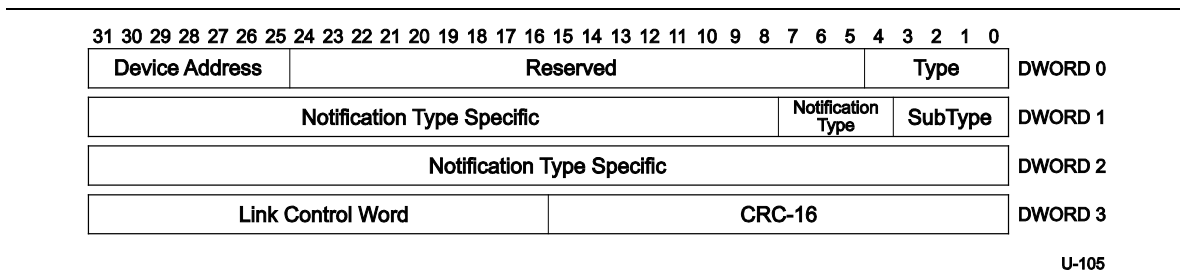
Figure 8-23. Device Notification Transaction Packet
