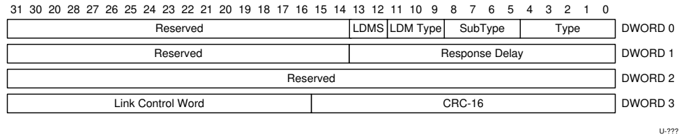
Figure 8-17. LDM LMP
