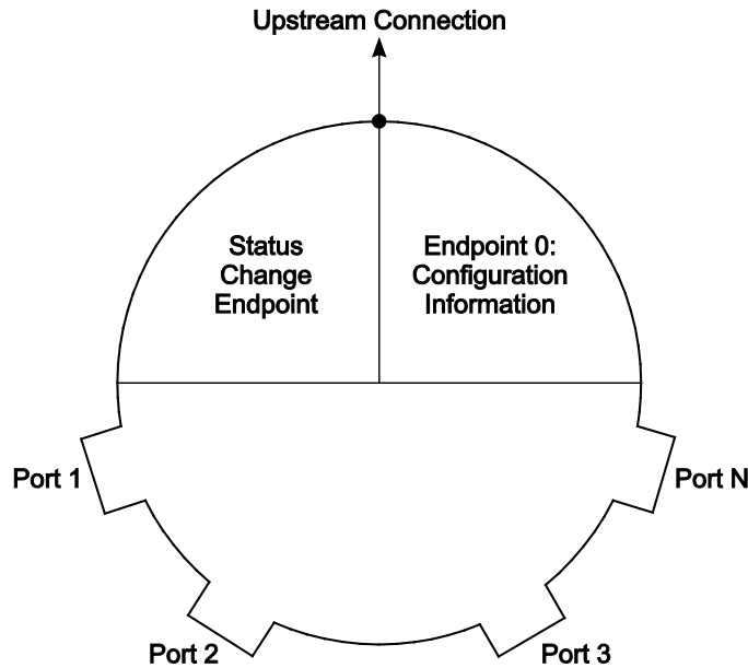
Figure 10-21. Example Hub Controller Organization
