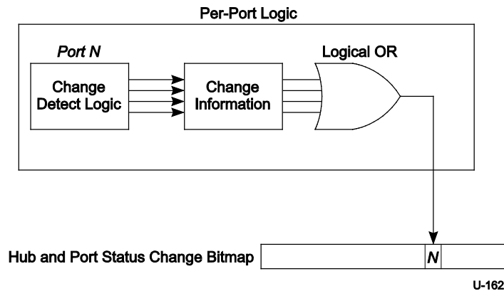
Figure 10-25. Example Hub and Port Change Bit Sampling
