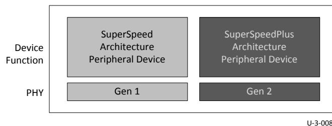
Figure 3-7. Enhanced SuperSpeed Device Configuration
