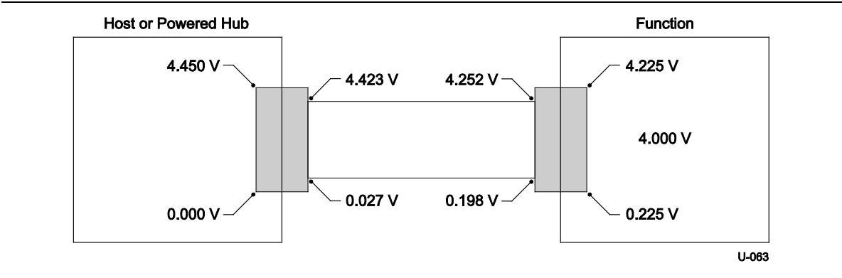
Figure 11-5. Worst-case Voltage Drop Topology (Steady
