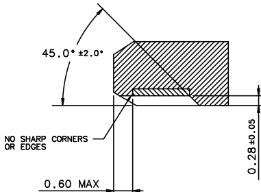
DETAIL Z
