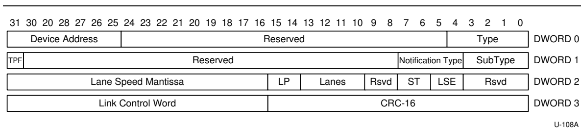
Figure 8-27. Sublink Speed Device Notification
