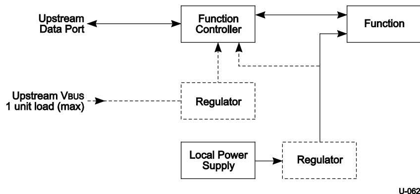
Figure 11-4. Self-powered Function
