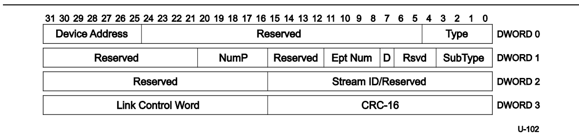
Figure 8-20. ERDY Transaction Packet
