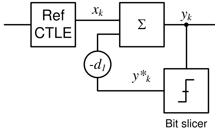
Figure 6-26. Gen 2 reference DFE Function
