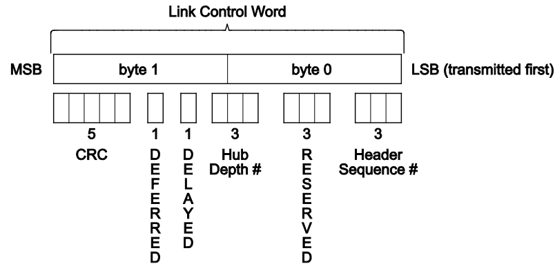
Figure 7-7. Link Control Word
