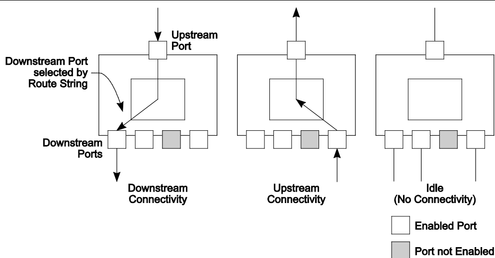
Figure 10-6. SuperSpeed Hub Signaling Connectivity
