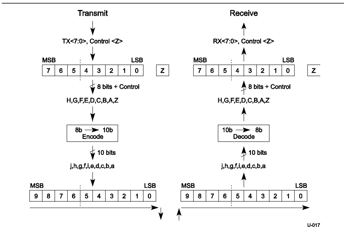
Figure 6-6. Character to Symbol Mapping
