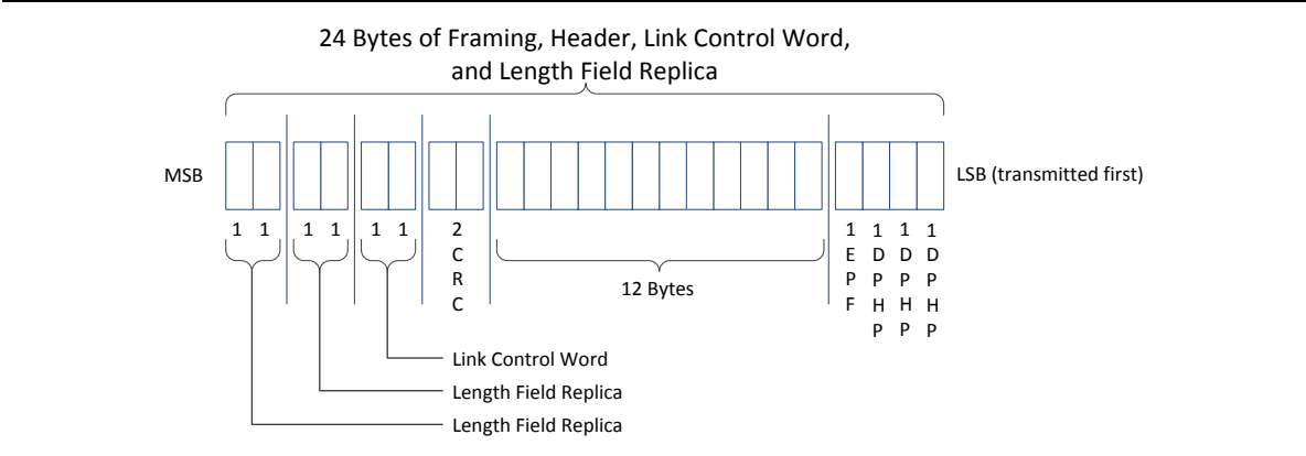
Figure 7-4. SuperSpeedPlus DPH Format
