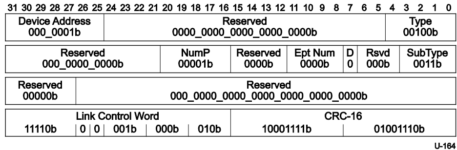
Figure D-1. Sample ERDY Transaction Packet
