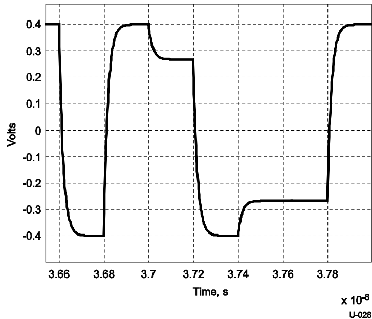
Figure 6-20. De-Emphasis Waveform
