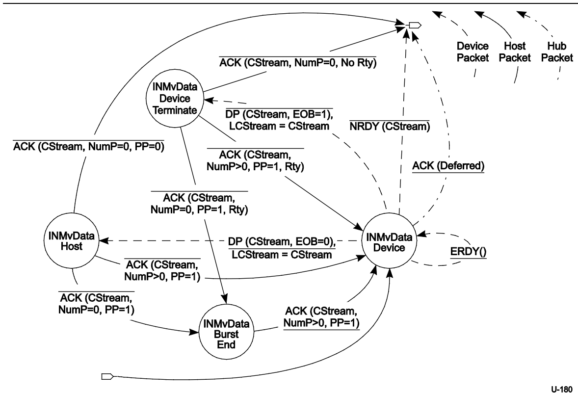
Figure 8-44. Host IN Move Data State Machine (HIMDSM)
