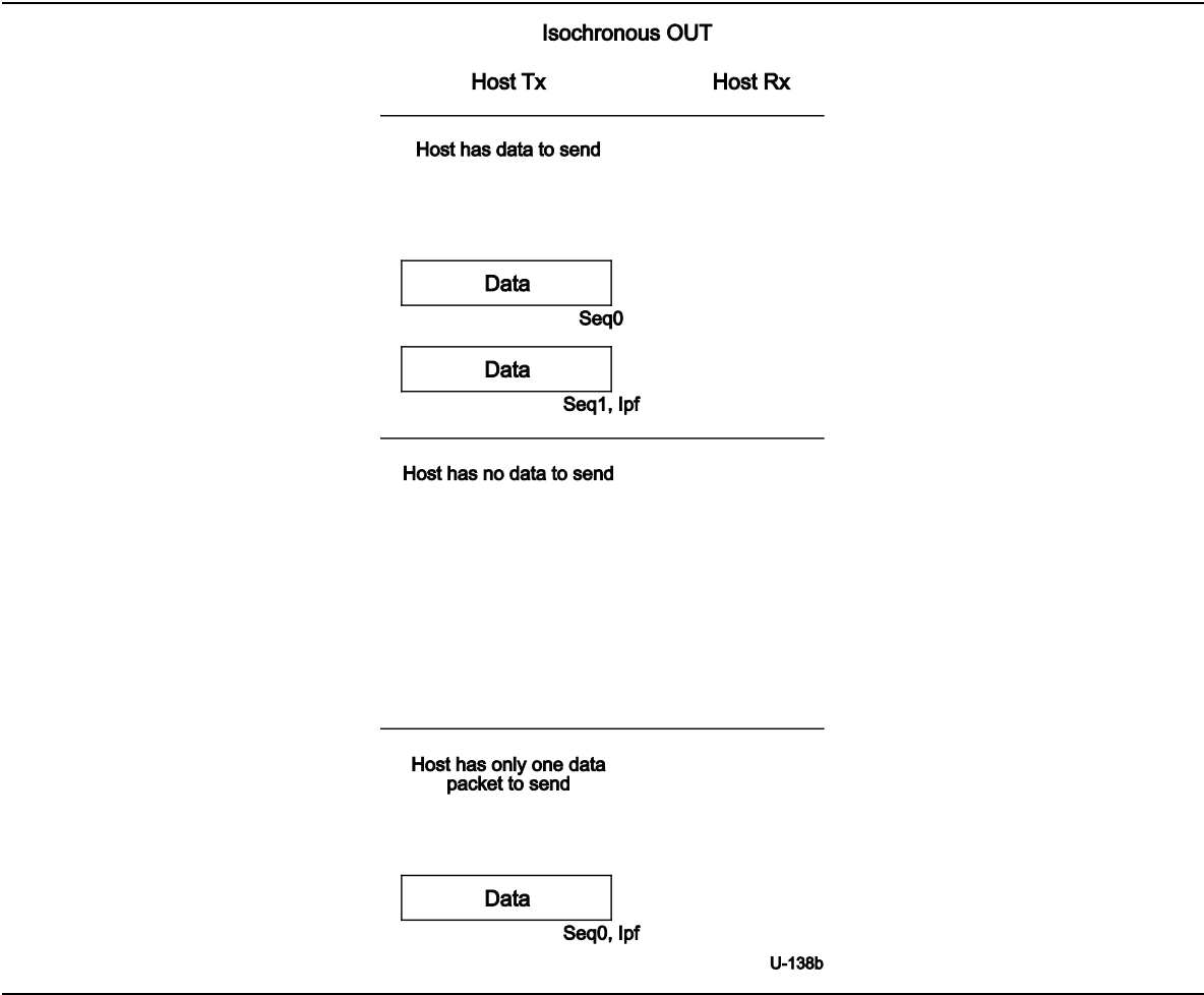
Figure 8-63. Sample Enhanced SuperSpeed Isochronous OUT Transaction
