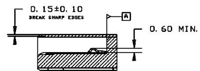
SECTION P-P
